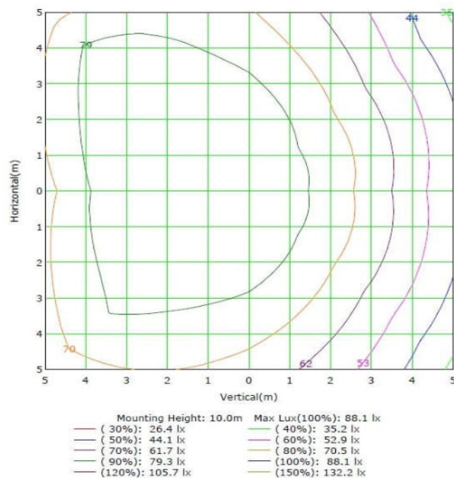
IsoLux Plot
