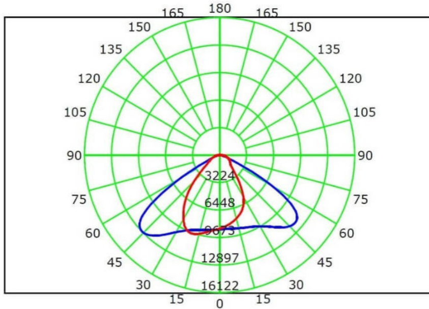
Luminous Intensity Distribution Curve
