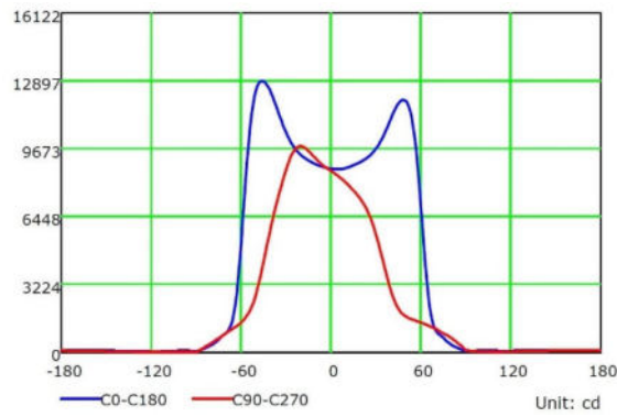
Isocandela (rectangle)
