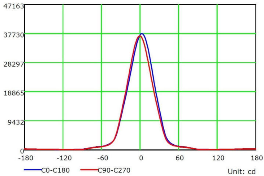
Isocandela (rectangle)
